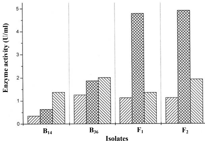
Fig. 3. Induction of \alpha -amylase. Cells were grown in the presence of 1% glucose (▨) and then shifted to minimal medium containing 0.5% starch (▩) or maltose (▧) as sole carbon source. Supernatants were collected and used as enzyme preparations to assay for \alpha -amylase activity. Isolates B 14 and B 36 are bacteria and F 1 and F 2 are fungi.
