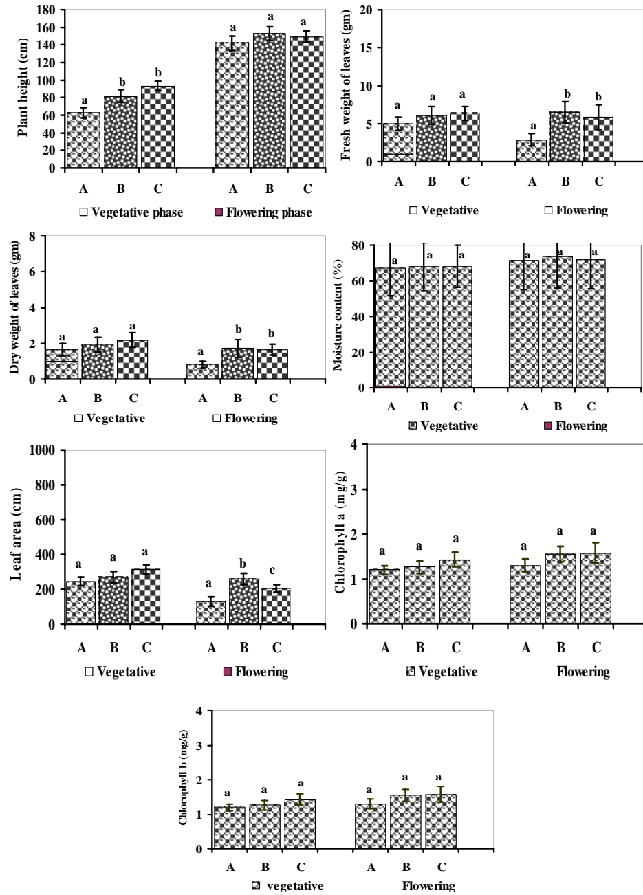
Fig. 1. Effect of treated wastewater on the growth of sunflower plant; A= fresh water (control); B= freshwater plus basal fertilizer urea, CaHPO 4 ·H 2 O, K 2 SO 4 ; C= treated wastewater.
