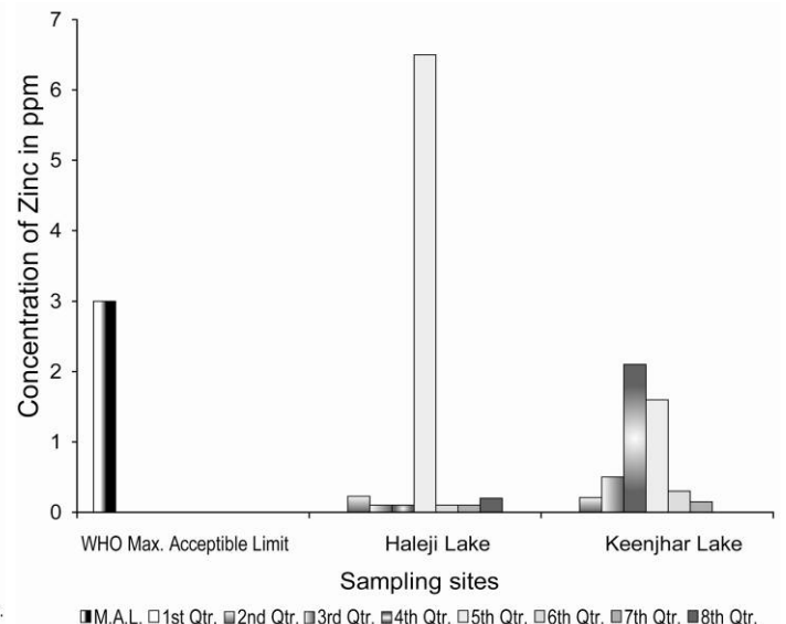
Fig. 3h. Zinc in water samples of Haleji and Keenjhar lakes.
