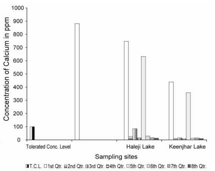
Fig. 5a. Calcium in fish samples of the two lakes.
