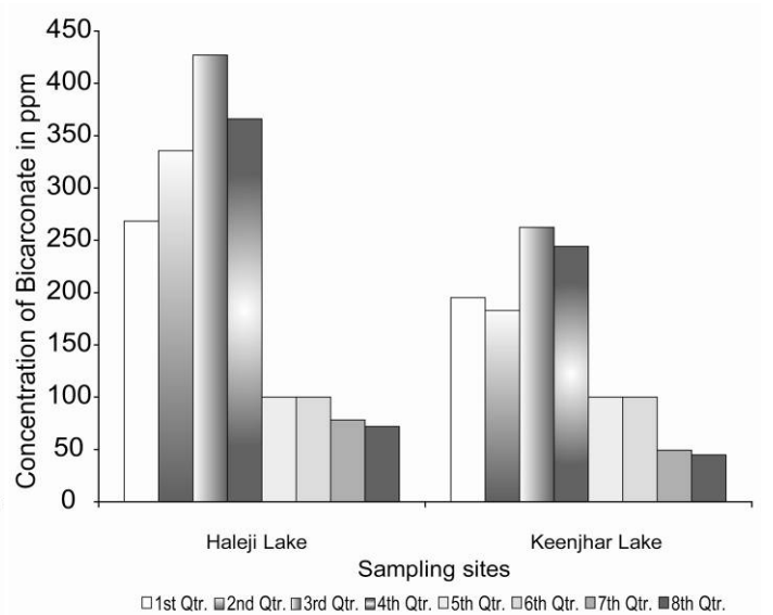
Fig. 4a. Bicarbonate in water samples of Haleji and Keenjhar lakes.
