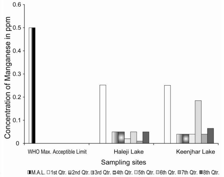
Fig. 3f. Manganese in water samples of Haleji and Keenjhar lakes.
