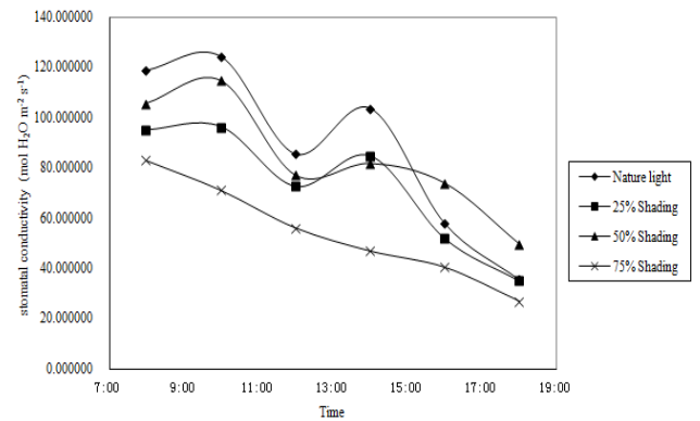
Fig. 6. The stomatal conductivity of tree peony 'FengDan'.
