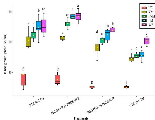
Fig. 5. Rice grain yield (mean of two years) as influenced by the interaction effect of various tillage practices and organic weed management (N=120) *Refer Table 1 for treatment details, The means with distinct letters within the same parameter indicate statistical significance, while identical letters denote non-significant at p \leq 0.05 .
