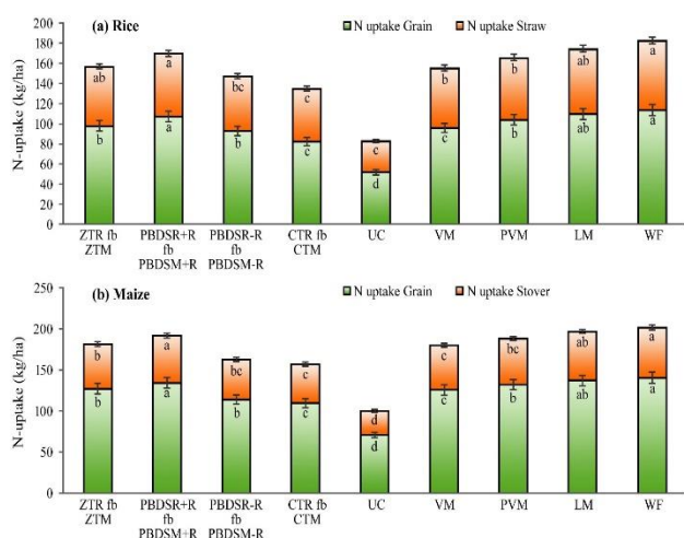
Fig. 4. N uptake (mean of two years) in grain and straw/stover of rice and maize as influenced by different tillage practices and organic weed management. *Refer Table 1 for treatment details, the means with distinct letters within the same parameter indicate statistical significance, while identical letters denote non-significant at p \leq 0.05 .
