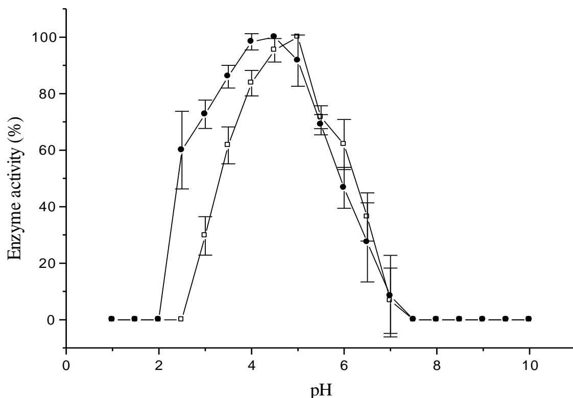
Fig. 3. Effect of pH on endoglucanase (□-) and β-glucosidase (●-) activity.
