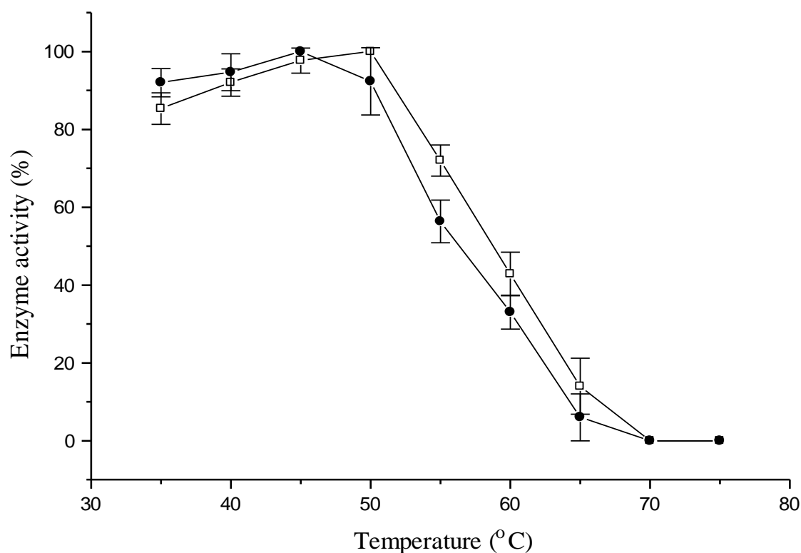
Fig. 2. Effect of temperature on endoglucanase (□-) and β-glucosidase (●-) activity.
