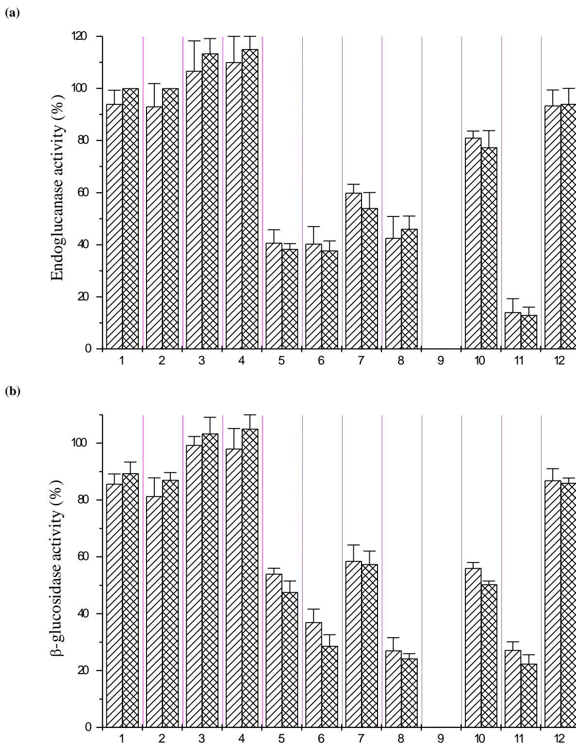
Fig. 4. Effect of metallic ions and EDTA on enzymes activity.
