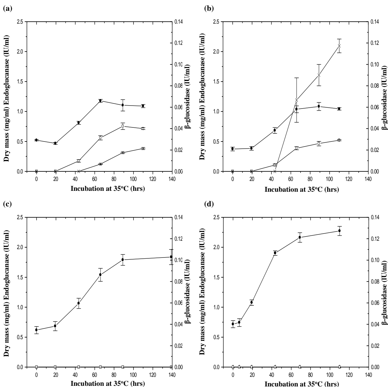
Fig. 1. Kinetics of Biomass (■), endoglucanase (□) and \beta -glucosidase (x) production in mineral salt medium containing (a) CMC (b) Salicin and (c) Glucose and in (d) SDB.
