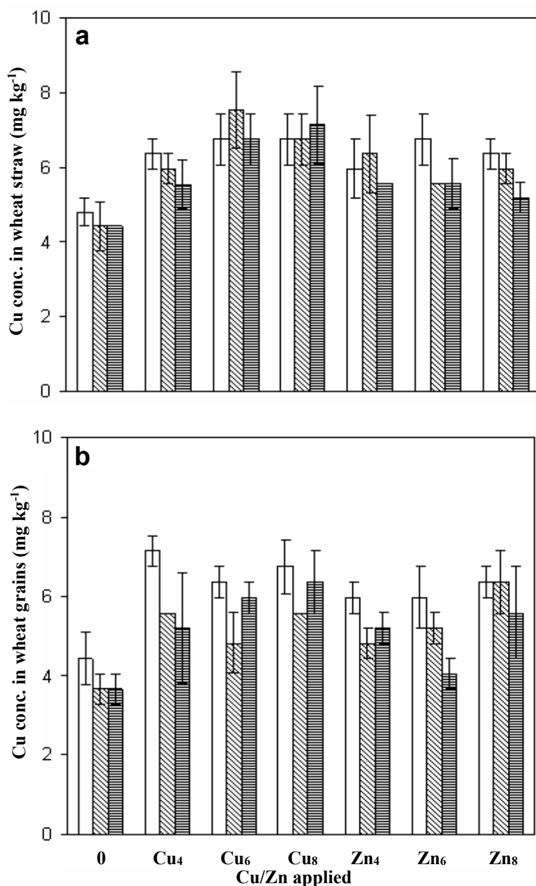
Fig. 2. Effect of texture, Cu and Zn application on Cu concentration in wheat: a) Straw and b) Grains.
