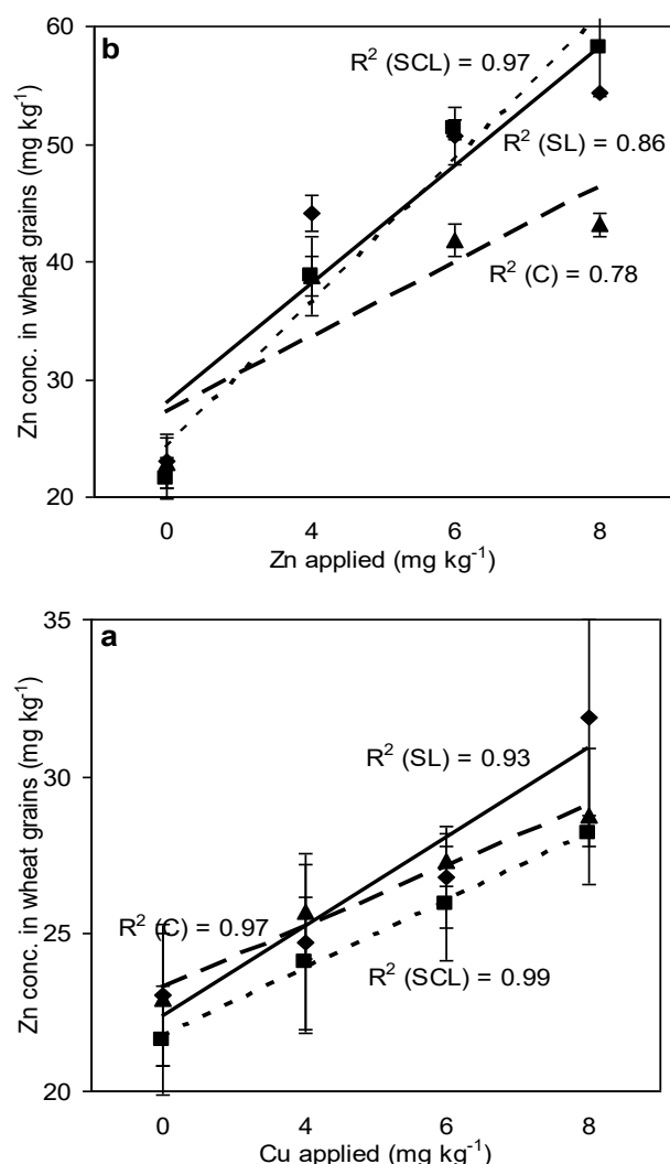
Fig. 4. Zn concentration in wheat grains influenced by soil texture and Cu/Zn application: a) effect of Cu applied, b) effect of Zn applied. [SL (◆)-Sandy loam; SCL (■)-Sandy clay loam; C (▲)-Clay].
