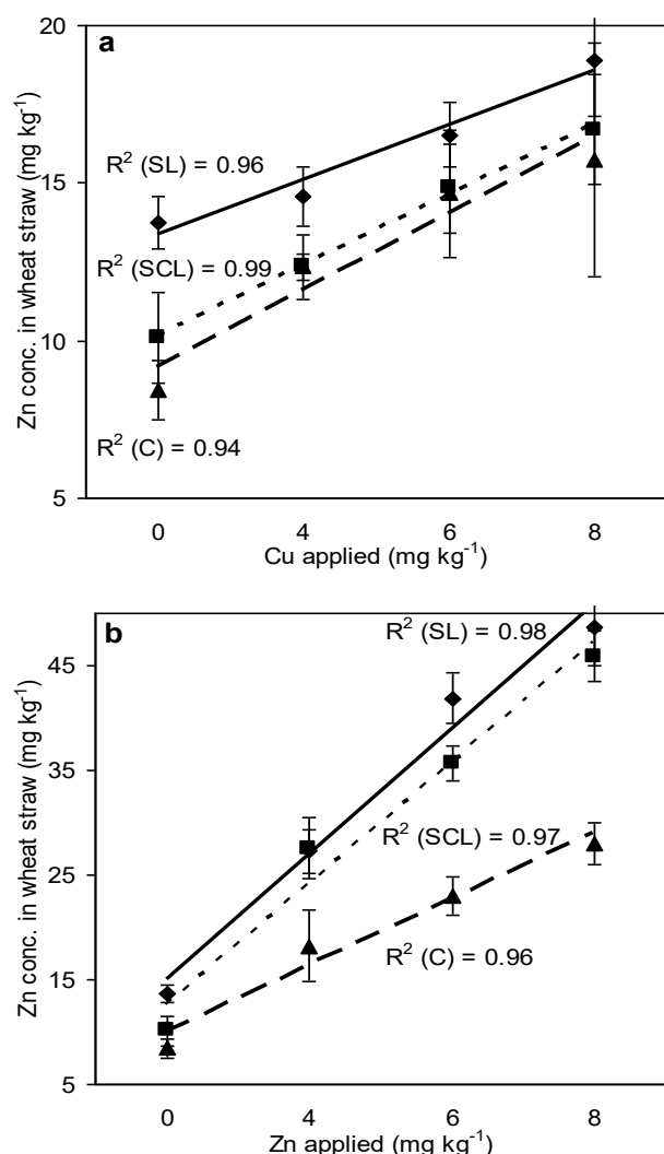
Fig. 3. Zn concentration in wheat straw influenced by soil texture and Cu/Zn application: a) effect of Cu applied, b) effect of Zn applied. [SL (◆)-Sandy loam; SCL (■)-Sandy clay loam; C (▲)-Clay].
