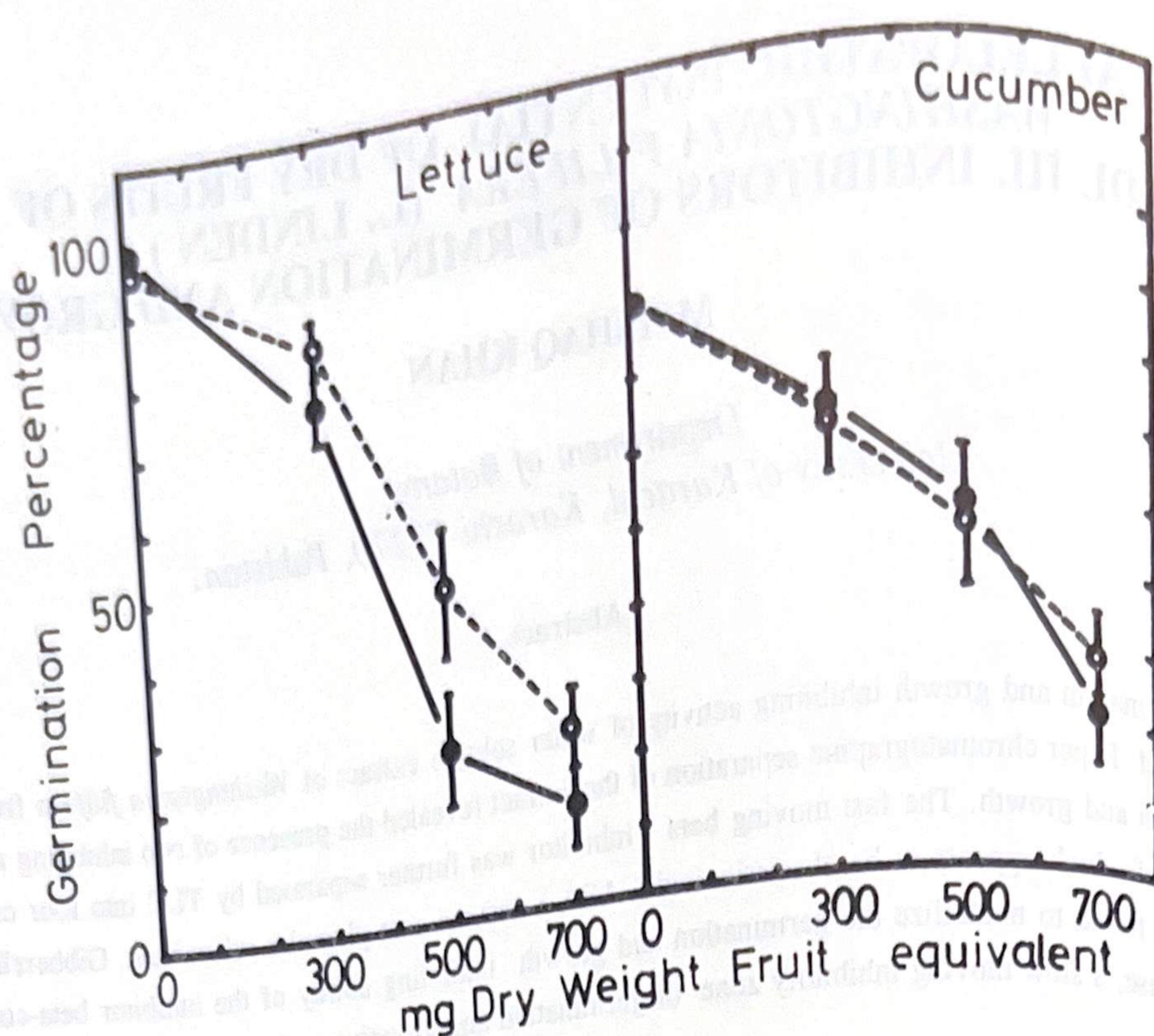
Fig.1. Effect of water-soluble extract of Washingtonia filifera fruits on lettuce and cucumber seed germination. Amount of water soluble (*-...*) and methanol soluble (*-...*) extract equivalent to 300, 500 and 700 mg dry weight of the fruit was used for the germination test. The vertical bars give standard error of the mean.
