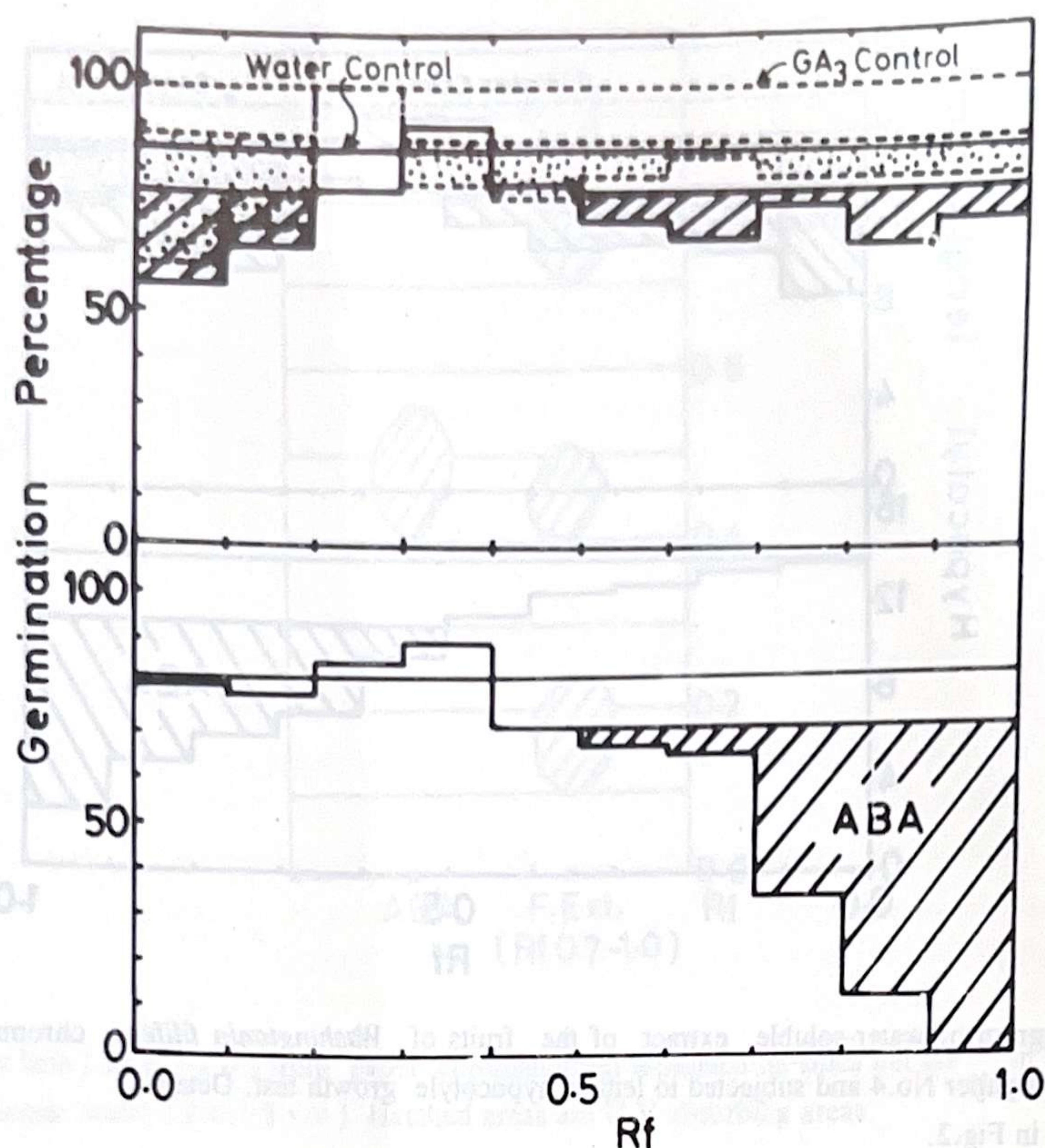
Fig.2. Histogram of water - soluble extract of the fruits of Washingtonia filifera chromatographed on Whatman paper No.4 in isopropanol: ammonia: water (10:1:1 v/v). Paper chromatograms were divided into ten equal pieces, placed in 9 cm Petri dishes and moistened with 2 ml of either distilled water or 10-ppm Gibberellic acid solution and 100 lettuce seeds were sown. Abscissic acid was also separated on paper and subjected to lettuce seed germination test. Hatched areas are significantly different ( p < 0.05 ) from the control.
