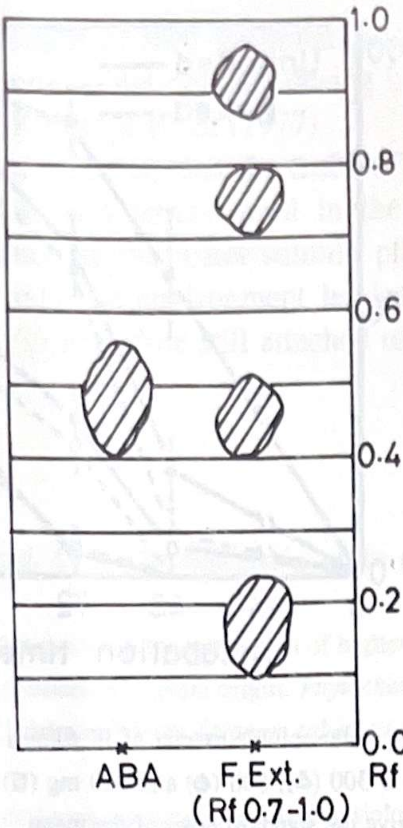
Fig.4. Inhibitor beta ( Rf 0.7-1.0 ) from paper chromatogram separated on silica gel HF 254 in n-butanol: n-propanol: ammonia: water ( 2:6:1:2 v/v ). Hatched areas are U.V absorbing areas.
