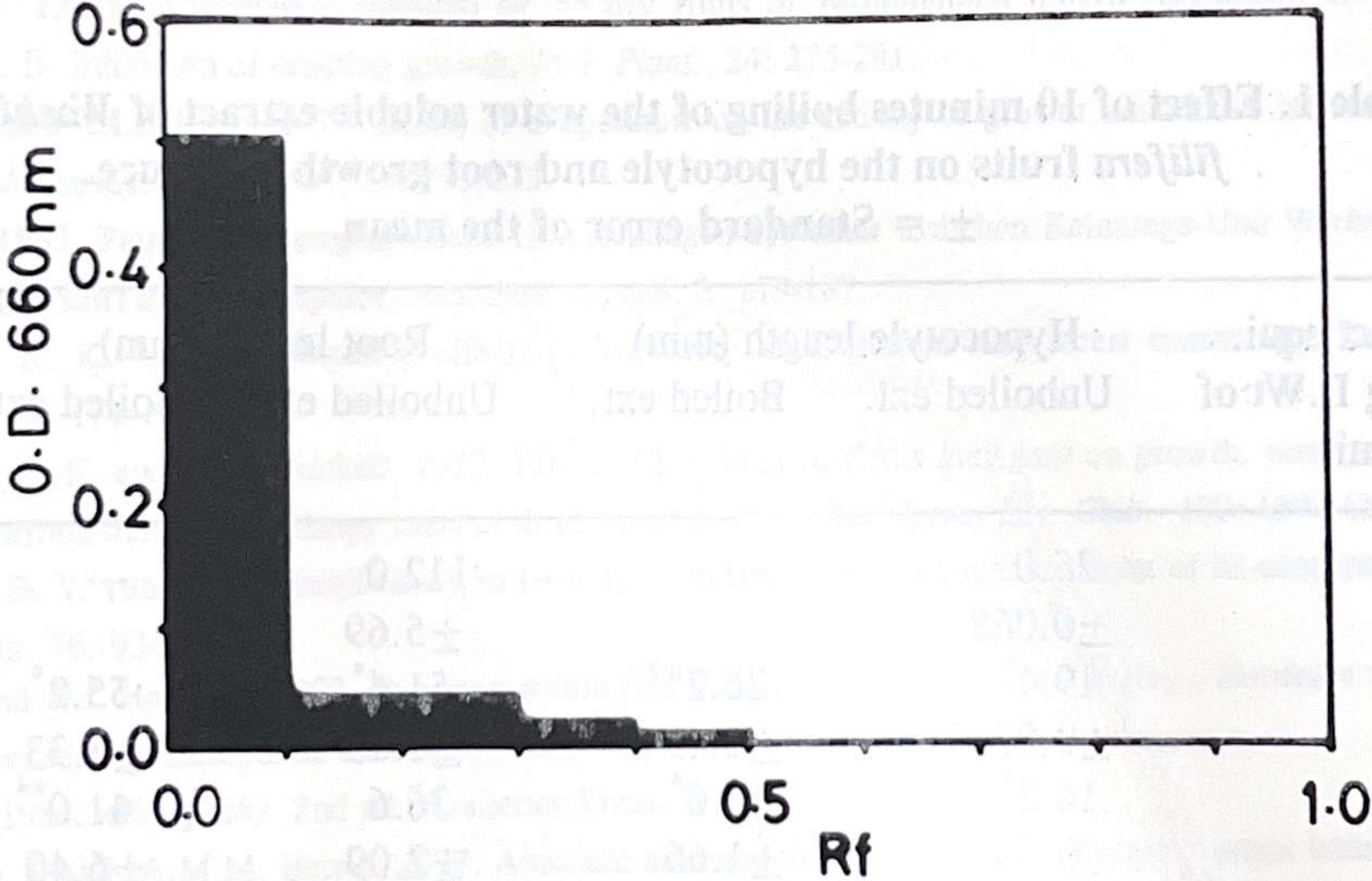
Fig.5. Chromatogram of slow moving inhibitory zone of water soluble extract of Palm fruit ( Rf 0.0-0.5 ) subjected to ascending paper chromatography with n-butanol: acetic acid: water (6:1:2 v/v). Paper divided into ten pieces,extracted with 50% ethanol and total phenol estimated at 660 nm.
