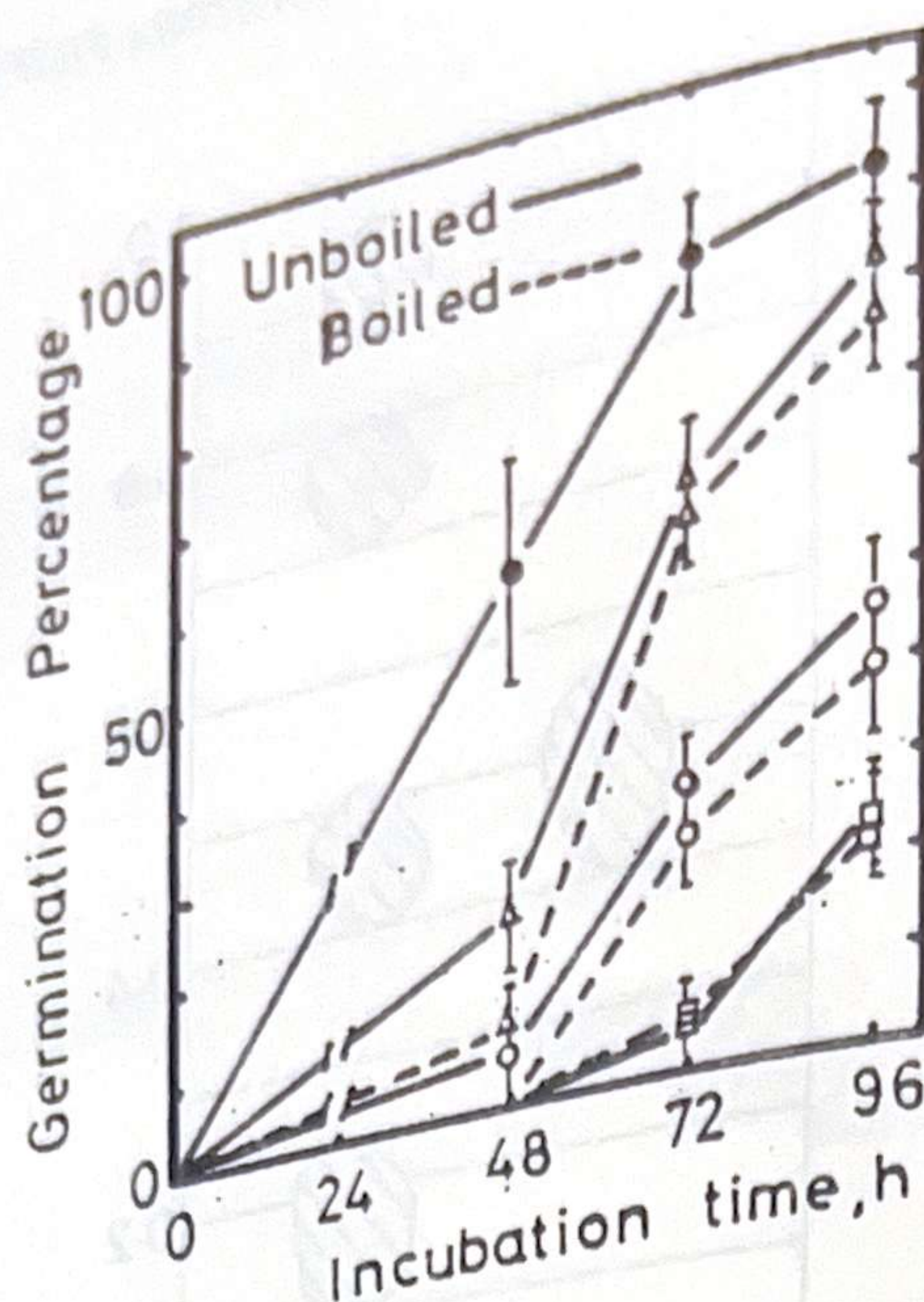
Fig.6. Effect of 10 min boiling of the water-soluble extract of W. filifera fruits on the germination of lettuce seeds. Amount of extract equivalent to 300 ( \Delta ), 500 ( \bullet ) and 700 mg ( \square ) dry weight of the fruits. Untreated water control ( \bullet ). The vertical bars give the standard error of the mean.
