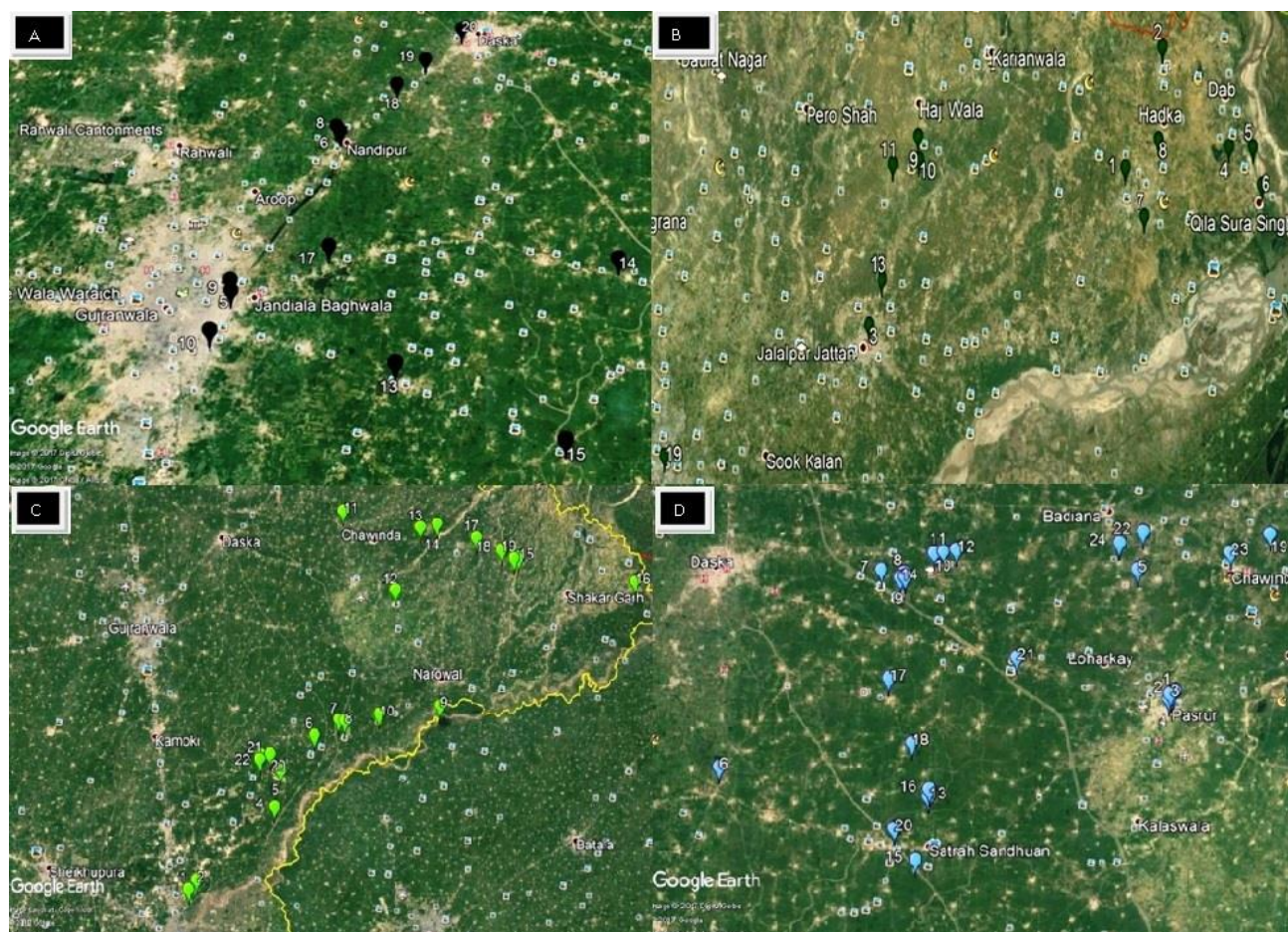
Fig. 1. Geographical positions of sampling units in four districts (A-D) of North East Punjab, Pakistan. (A: Gujranwala, B: Gujrat, C: Narowal, D: Sialkot)
