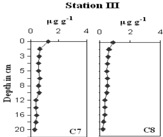
Fig. 2. Vertical profile of Chl a in sediments at Station III. Each point is a mean of duplicate values.
