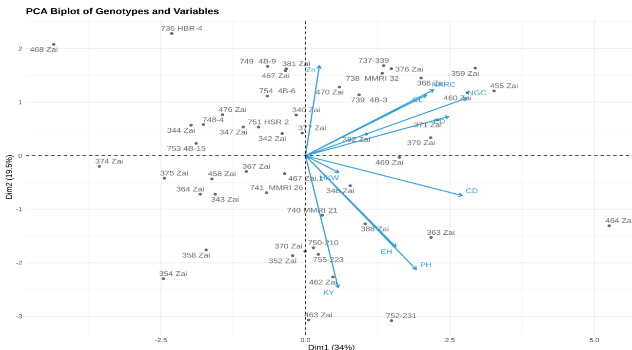
Fig. 4. PCA Biplot of morphological and biochemical traits of maize inbred lines ED= Ear diameter (cm), CL= Cob length (cm), NKRC= Number of kernel rows per cob, NGC= Number of grains per cob, PH= Plant height (cm), HKW= Hundred kernel weight (g), CD= Cob diameter (cm), KY= Kernel yield (g), Zn= zinc (ppm), and EH= Ear height (cm)
