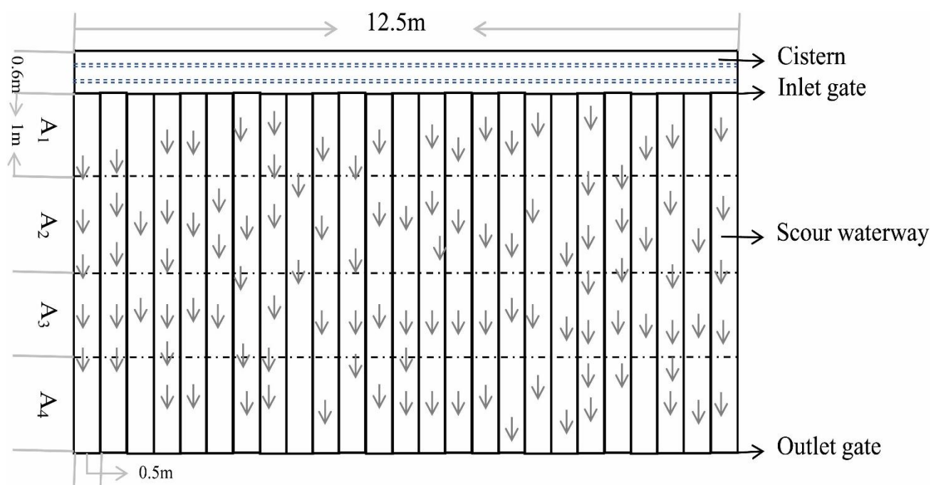
Fig. 1. Schematic diagram of experiment site.
