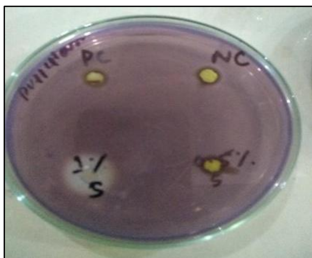
Fig. 6. Activities of amylolytic enzymes observed on pullulan agar plate treated with diluted Gram's iodine.
