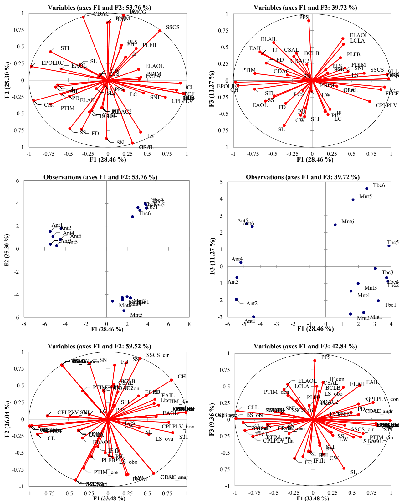
Fig. 2. Labels: A, B and E: Plant: Length of stem: PLS, Plant: Height: PG, Plant: Density: PD, Flower position compared to foliage: FPCF, Stem: Number of internodes: SNI, Plant: Laterals with flower buds or flowers of second order: PLFB, Plant: Clustering on lateral branches: BCLB, Inflorescence: form: IF, Stem: Length of internode: SLI, Stem thickness of internode: STI, Stem shape in cross section: SSCS, Leaf Shape: LS, Leaf length: LL, Leaf width: LW, Leaf: curvature of longitudinal axis: LCLA, Leaf Cross Section: LCS, Leaf color: LC, Bud: shape: BS, Epicalyx: Position of outer lobes in relation calyx: EPOLRC, Epicalyx: apex of outer lobes: EAOL, Epicalyx: apex of inner lobes: EAIL, Epicalyx: Length of apex of inner lobes: ELAIL, Calyx: Length: CL, Calyx: width: CW, Calyx: Longitudinal axis of lobes: CLAL, Calyx: Distribution of Anthocyanin coloration: CDAC, Calyx: Distribution of Anthocyanin coloration: CDAC2, Calyx: shape of apex of lobes: CSAL, Calyx: Length of lobes, Flower: Diameter: FD, Corolla Height: CH, Corolla: Profile of lower part in lateral view: CPLPLV, Petals: Predominant shape: PPS, Petals undulation: PU, Petals: Number of incisions of margin: PNIM, Petal: type of incisions of margin: PTIM, Petals: Depth of incision of margins: PDIM, Petal: Main color Group: PMCG, Ovary shape: Osp, Ovary: color of base: OCB, Ovary Surface: OSrf, Style: Number: SN, Style: Length: SL Style: Shoulder: SS, Stigma: color: SC. C, D and F: Ant: Antigua, Mnt: Montoyo and Tbc: Tabasco.
