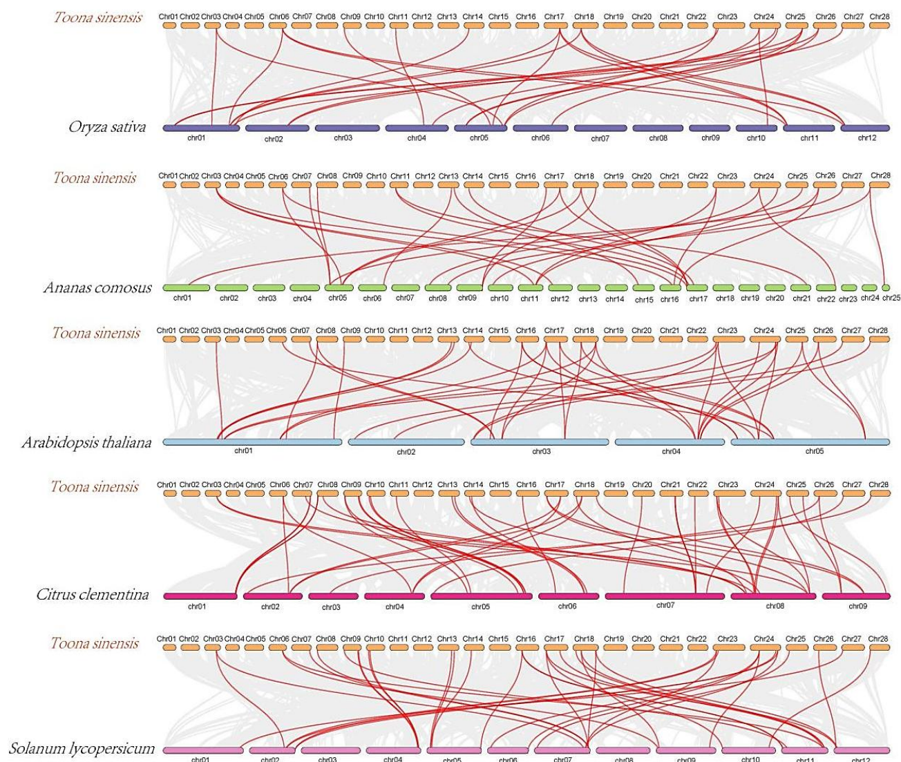
Fig. 6. Synteny analysis of NAC genes between T. sinensis and five typical plants: Ananas comosus ( A. comosus ), Oryza sativa ( O. sativa ), Arabidopsis thaliana ( A. thaliana ), Citrus clementina ( C. clementina ), and Solanum lycopersicum ( S. lycopersicum ). The red curves indicate the syntenic NAC gene pairs, whereas the gray lines represent the collinear blocks of T. sinensis and other plants.
