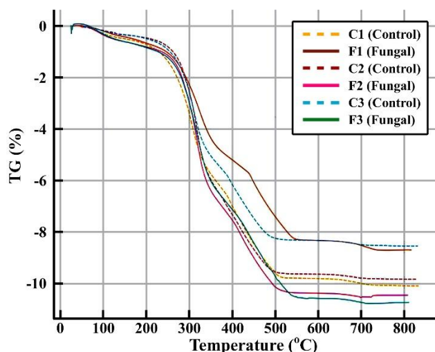
Fig. 5. TGA Analysis.
