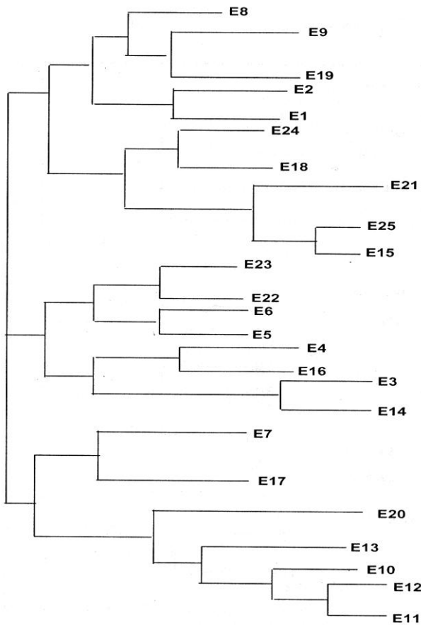
Fig. 4. Dendrogram of 25 Sea Buckthorn Ecotypes.
