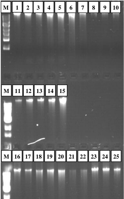
Fig. 2. Genomic DNA of sea buckthorn ecotypes.
