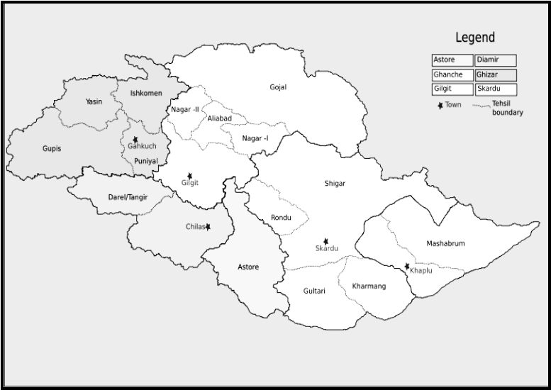
Fig. 1. Sampling sites from Northern areas of Pakistan.
