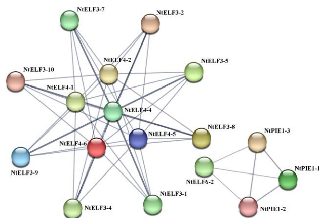
Fig. 6. Protein-protein interaction network of NtELF family proteins. (The thickness of the line segment represented the strength of the interaction).
