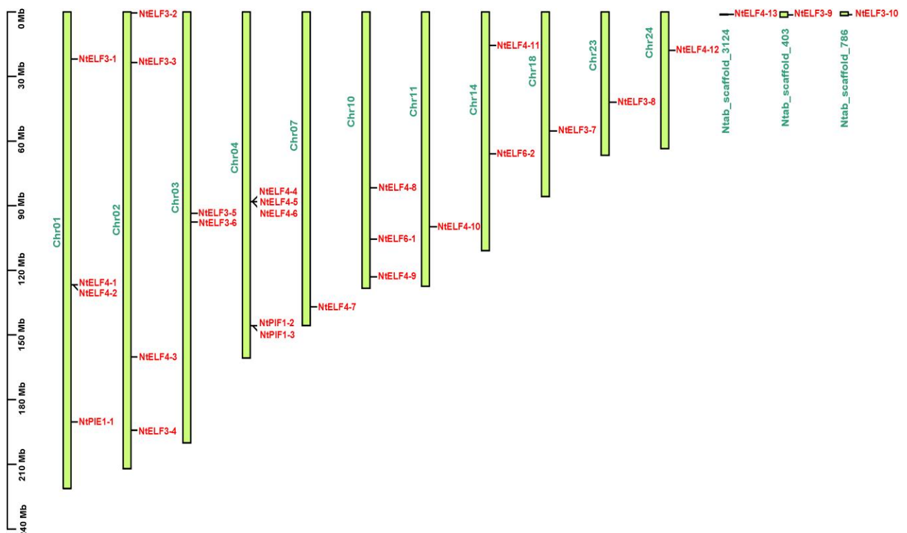
Fig. 2. The location of NtELFs . The green column indicated the chromosomes of N. tabacum , and its length indicated the chromosomes length).
