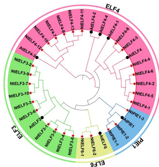
Fig. 1. Phylogenetic tree of ELF family in Nicotiana tabacum and Arabidopsis thaliana (Different colors on the rings indicated different subfamilies. Members of the A. thaliana family were represented by dots, and members of N. tabacum family were represented by five-pointed stars).
