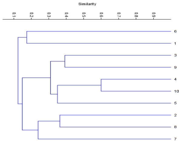
Fig. 13. The dendrogram of the connections between the study stations. 1: Juwaibdah 2: Hartha 3: Jabal Sanam 4: Khader Al-May 5: Um-Qaser 6: South Rumaila 7: Zariji 8: Qarmat Ali 9: North Rumaila 10: Jrishan.
