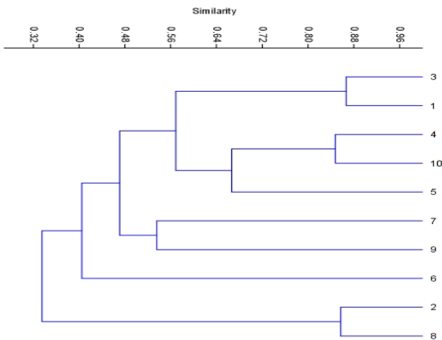
Fig. 14. The dendrogram of the connections between the study stations. 1: Juwaibdah 2: Hartha 3: Jabal Sanam 4: Khader Al-May 5: Um-Qaser 6: South Rumaila 7: Zariji 8: Qarmat Ali 9: North Rumaila 10: Jrishan
