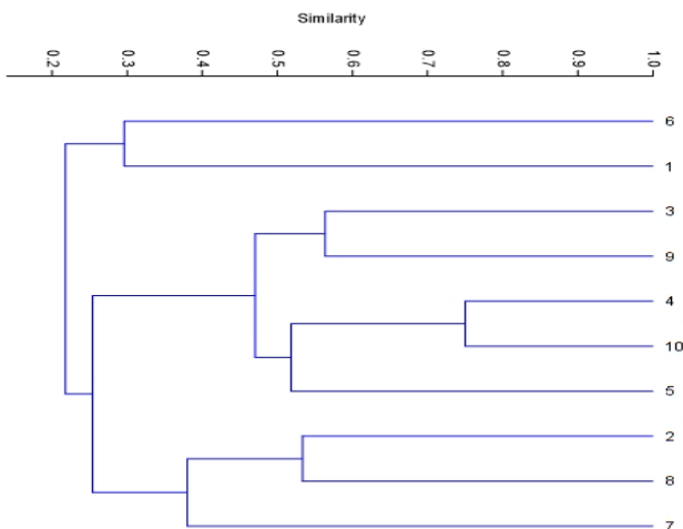
Fig. 15. The dendrogram of the connections between the study stations 1: Juwaibdah 2: Hartha 3: Jabal Sanam 4: Khader Al-May 5: Um-Qaser 6: South Rumaila 7: Zariji 8: Qarmat Ali 9: North Rumaila 10: Jrishan
