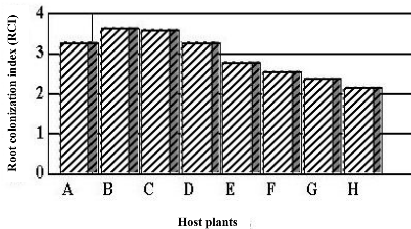
Fig. 2. Root colonization by Sclerotium rolfssii on different test plants in soil artificially infested with S. rolfssii @ 1 sclerotium \text{g}^{-1} soil.
