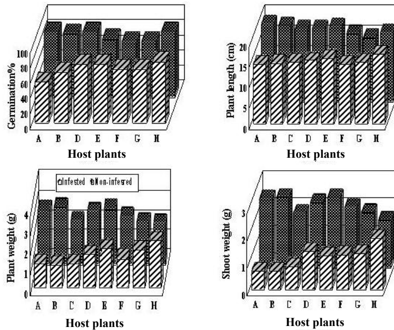
Fig. 1. Effect of Sclerotium rolfssii on growth of different test plants.
