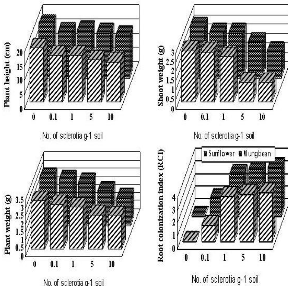
Fig. 3. Effect of different population levels of Sclerotium rolfii on plant growth and root colonization of mungbean and sunflower.
